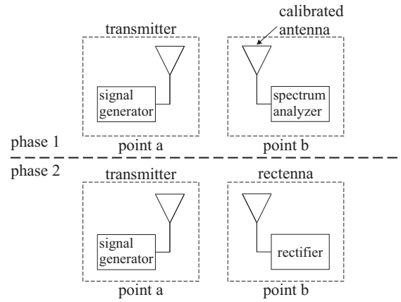
Fig. 9. The rectenna RF-to-dc efficiency measurement two-phase methodology.
