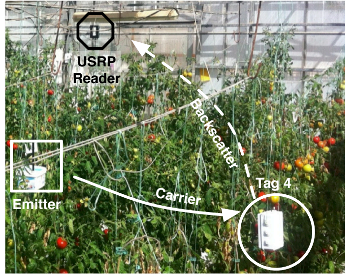
Fig. 14: Left: Experimental network topology. 10 %RH sensors, 1 plant voltage sensor and 2 carrier emitters with transmit power at 20 mW were deployed. Right: Photo of the deployment inside the greenhouse.
