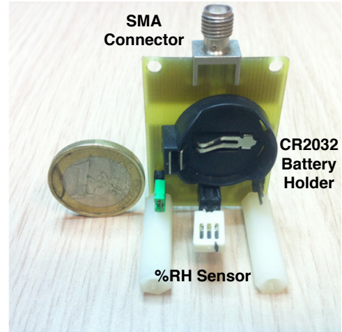
Fig. 4: The prototype sensor tag developed.
