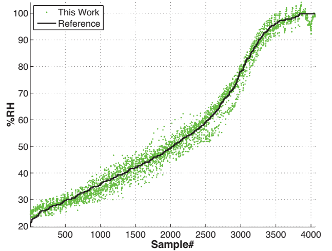
Fig. 10: Reference vs received %RH measurements.
