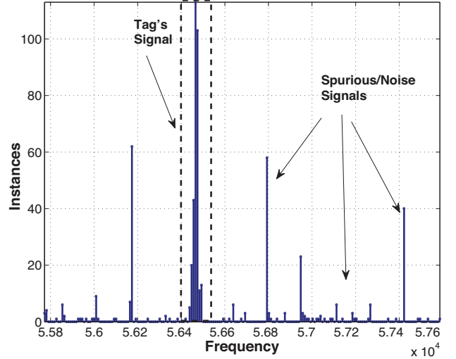
Fig. 12: Histogram filtering: A set of measurements is collected and their histogram is calculated. Only measurements within a certain range and with the highest occurrence are kept.
