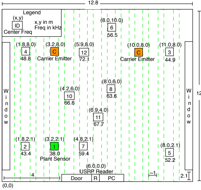
Fig. 14: Left: Experimental network topology. 10 %RH sensors, 1 plant voltage sensor and 2 carrier emitters with transmit power at 20 mW were deployed. Right: Photo of the deployment inside the greenhouse.
