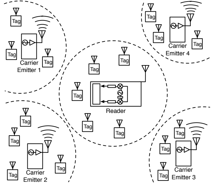
Fig. 6: Proposed WSN overview. Multiple, low-cost carrier emitters are placed in the field and around them, many ultra low-power tags are deployed.
