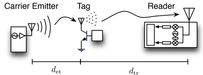
Fig. 2: Bistatic scatter-radio topology; carrier emitter placed in a different location from the reader. d_{et} and d_{tr} denote the emitter-to-tag and tag-to-reader distance, respectively.
